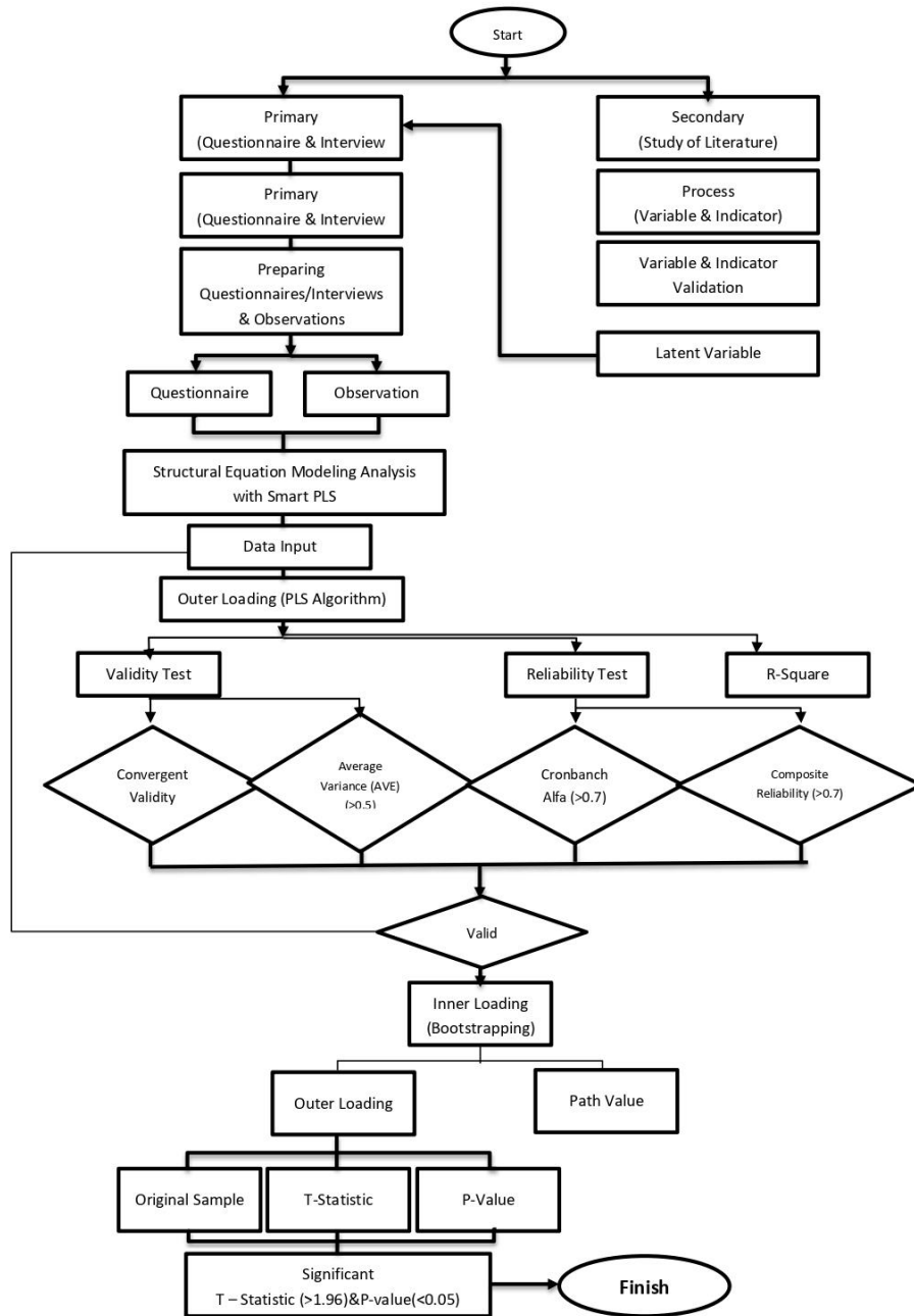
Fig. 3. Data Processing Diagram with SEM-PLS Source: processed by Author
