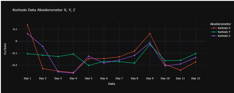
Fig. 12. Kurtosis Data Accelerometer X, Y, Z
