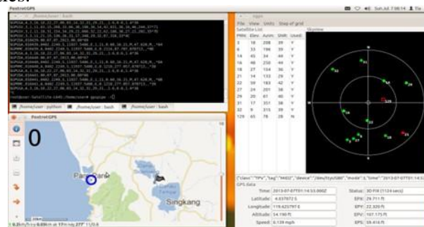
Fig. 6. NMEA Data, Satellite Conditions, and User Position on Parepare Beach Data Collection Map
