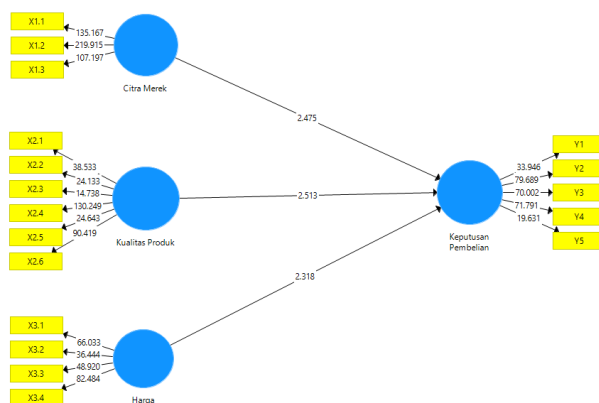
Gambar 2. Bootstrapping Test Results
